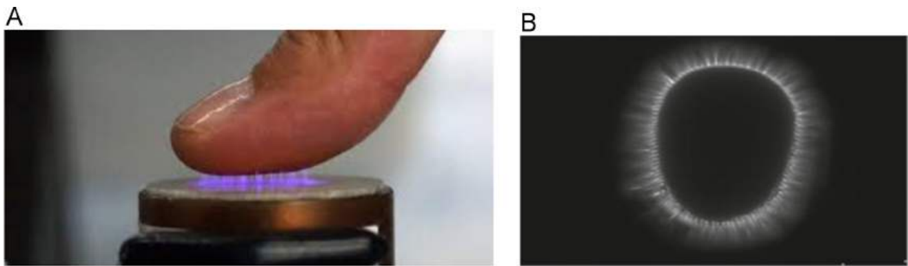
Figure 79: Biophotons. Source: [761].
