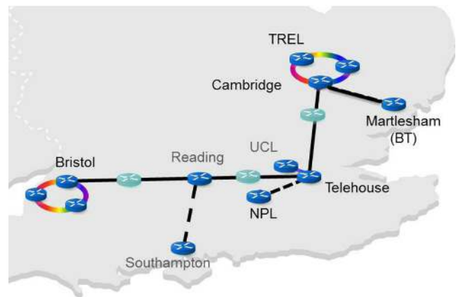
Figure 26: UK National Dark Fibre Infrastructure Service. Source: The Quantum Communications Hub, 2016 (11 slides).
