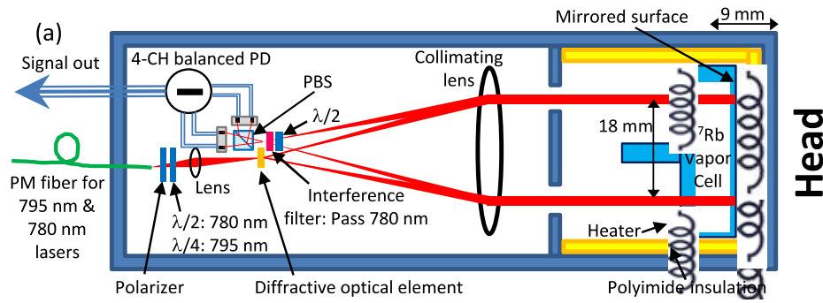
Figure 153: The principle of an OPM-based magnetoencephalography sensor. Source: [1467].
