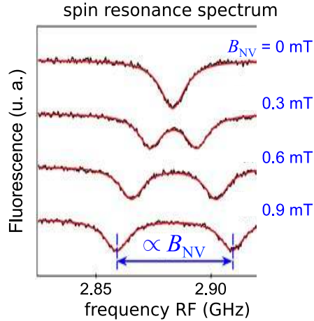
Figure 131: NV center static magnetometry principle using spin resonance spectrum analysis. The two energy gaps which depend on the ambient magnetic field enable the evaluation its current value. Source: [1303].
