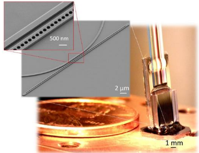
Figure 172: Quantum photonic thermometer from NIST.
