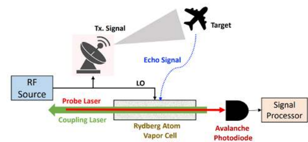
Figure 168: A Rydberg atom glass cell could help better amplify the incoming microwaves received by a classical radar. Source: [1522].
