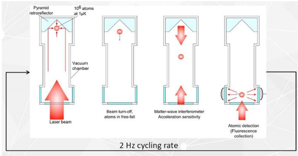
Figure 112: How atom interferometry works. All laser beams come from the bottom of the device. Source: Muquans.
