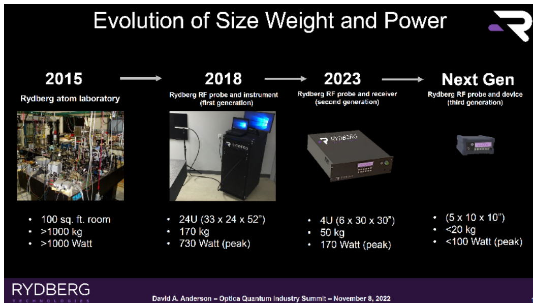
Figure 142: Rydberg Technologies miniaturization roadmap as presented at the Optica Conference in November 2022. Source: Rydberg Technologies. Added in 2023.
