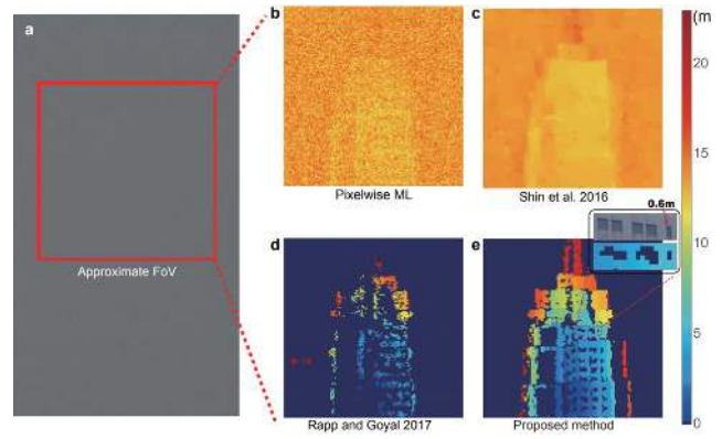
Figure 171: The simulated result of the 2019 quantum LiDAR. Sources: [1424, 1550].
