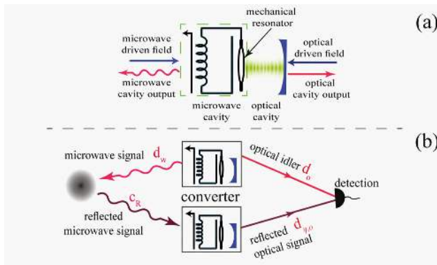
Figure 169: Converting radar RF waves to/from photons. Source: [1528].
