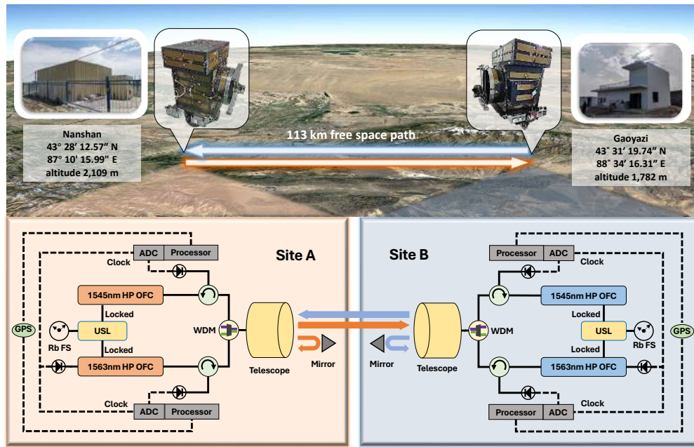
Figure 166: 113 km distance sensing implemented in China in 2024 with dual optical frequency combs. Source: [1499].
