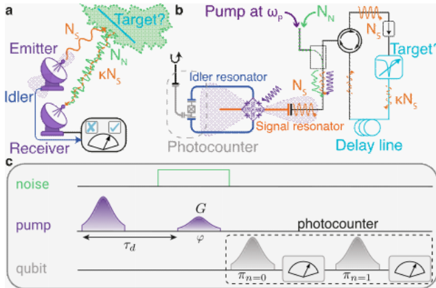
Figure 167: The superconducting circuitry based microwave quantum radar proposed by ENS Lyon in 2023, using a delay line. Source: [1514].
