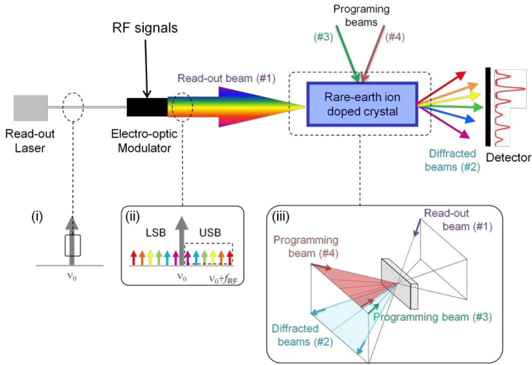
Figure 140: Spectral hole burning (SHB) RF sensing technique developed by Thales. It uses a “rainbow architecture” that starts with a RF signal conversion to optical wavelengths using a Mach-Zehnder electro-optical modulator driven by a laser and then, diffraction of the resulting optical beam by a rare-earth-ion-doped crystal cooled to 3 K, followed by detection with an array of photodetectors. It supports 20 GHz bandwidth with sub-MHz resolution. Source: [1386].
