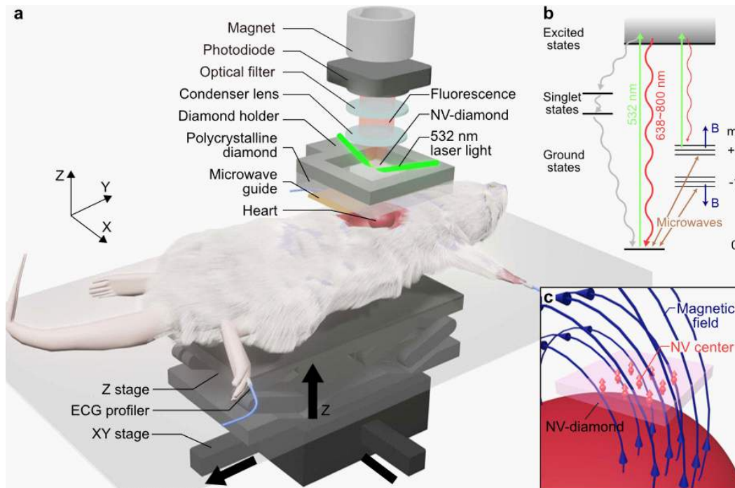
Figure 148: NV center based magnetocardiography experiment on rats. Source: [1457].
