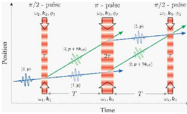
Figure 114: The three steps of cold atoms interferometry used in a gravimeter. Sources: [1236].
