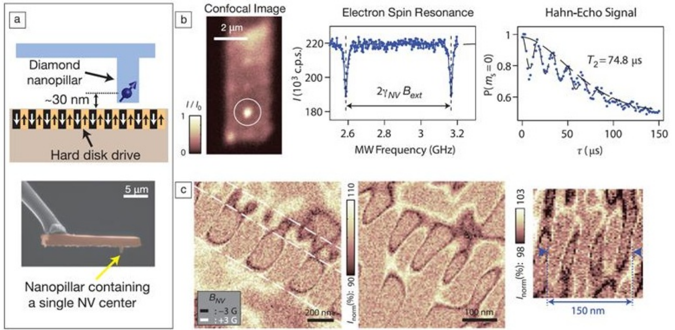
Figure 149: Schematic of a monolithic diamond nanopillar probe (top) and representative SEM image of the nanopillar probe (bottom). (b) Characteristics of a nanopillar probe device. Confocal image of the device (left) clearly shows a localized fluorescence spot from a single NV center at the position of the nanopillar. Electron spin resonance (middle) was acquired with an enhanced fluorescence of 220,000 photons/sec. The coherence time of the measured Hahn-echo signal (right) is 74.8 \mu\text{s} , an order of magnitude longer than a typical Hahn-echo coherence time of commercial diamond nanocrystals ( \sim 5 \mu\text{s} ). (c) Magnetic images of a hard disk drive acquired by the nanopillar probe. Alternating magnetic bits were imaged with varying sizes down to 25 nm (right), indicating the distance between a single NV center at the probe and the hard disk sample is roughly within 25 nm. Source: [1459].
