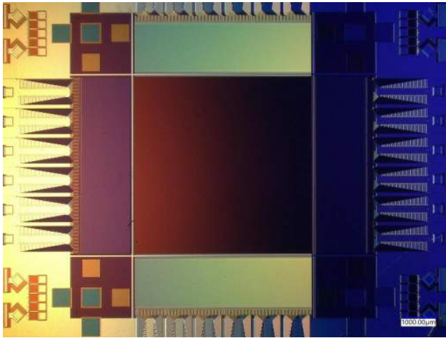
Figure 144: The 400,000-pixel SNSPD camera chip from NIST, developed in 2023. Source: NIST.
