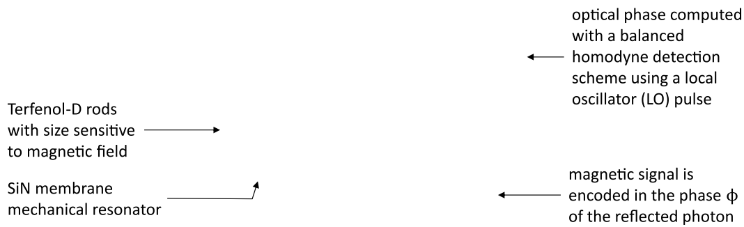
Figure 134: A SiN-based optomechanics-photonics magnetometry quantum sensor developed in China in 2022. Source: [1324].
