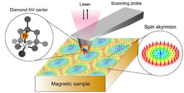
Figure 132: NV centers used in ODMR for medical imaging of materials inspection. Source: [1312].
