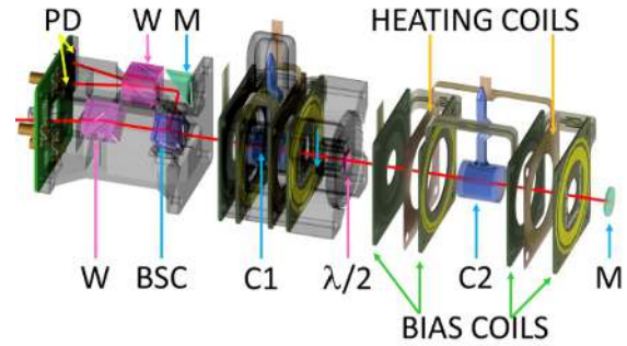
Figure 151: OPM based Magnetocardiography Sensor layout. The laser beam (red line) is delivered with an optical fiber and collimated using a GRIN lens (not shown). The beam is deflected on a Wollaston prism (W), 10% of the beam passes through the beam splitting cube (BSC), cell 1 (C1), half-wave plate ( \lambda/2 ), cell 2 (C2) and is retroreflected with a mirror (M). After passing through the cells the second time, 90% of the beam is reflected by the BSC and then a right-angle mirror to the polarimeter formed by a second Wollaston prism and two PDs. The coils surrounding both cells are identical but are expanded around C2 for better visualization. Source: [1468].
