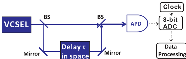
Figure 28: An APD (avalanche photodetector) operating principle. Source: [214].
