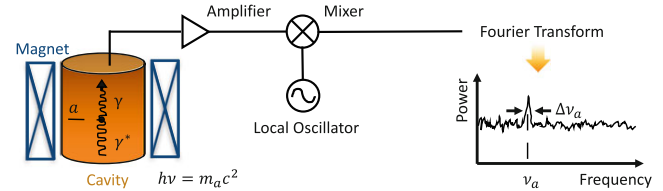
Figure 179: Simplified axion detection schematic of microwave cavity searches. Much like an AM radio, the high frequency axion signal is mixed down to audio frequencies by mixing with a local oscillator maintained at a fixed offset frequency from the cavity frequency. This allows for much lower digitization rates. The cartoon power spectrum shows a sample axion signal above the noise. Caption and schema source: [1606].
