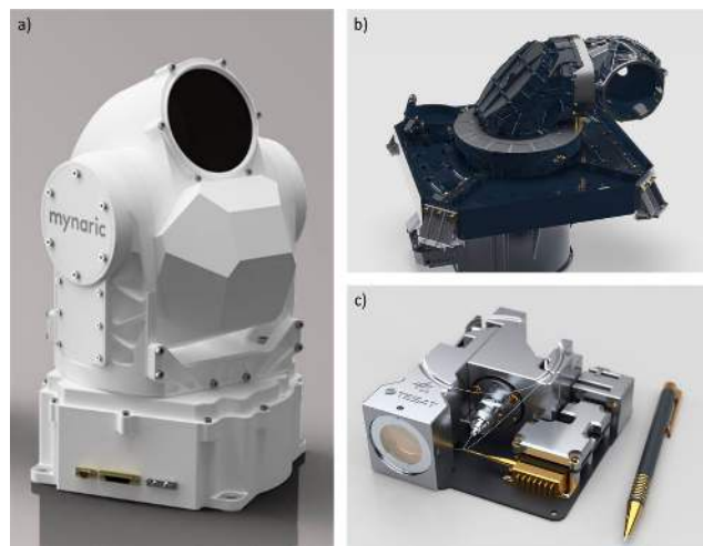
Figure 50: Examples of optical terminals for satellite-to-satellite and satellite-to-ground communication, including a Mynaric Condor MK3 ground station (a), a Coarse Pointing Assembly (CPA) from Tesat (b), and a satellite optical module (c). Source: [452].
