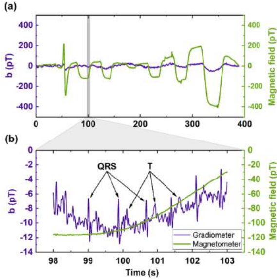
Figure 152: The signal output of the OPM based Magnetocardiography Sensor with the difference between the magnetic field and the more precise magnetic gradiometer field. The chart in (a) covers the full duration of the recording while (b) zooms on a specific period. The purple trace is the gradiometer signal and the green trace is the reference magnetometer showing the magnetic field component in the gradiometer's sensitive axis direction. At 50 s, the impact of a magnetic door lock as a door is opened and closed is visible. After 70 s, the operation of the building's lifts started. The arrows indicate the QRS complex and T wave of the measured heartbeat. Source: [1468].
