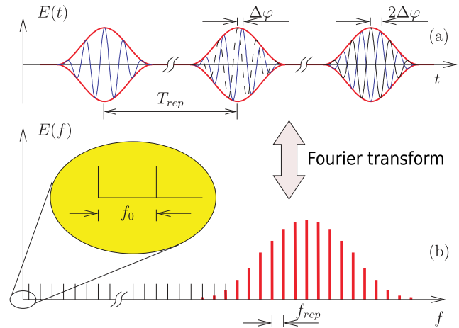
Figure 121: How a frequency comb works. Source: Ultra-short light pulses for frequency metrology , CNRS (6 pages).
