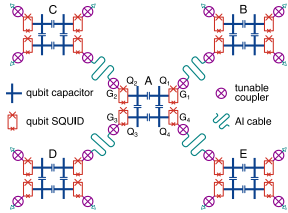
Figure 65: The five-superconducting-chip layout implementing short-range connectivity. Source: [807].
