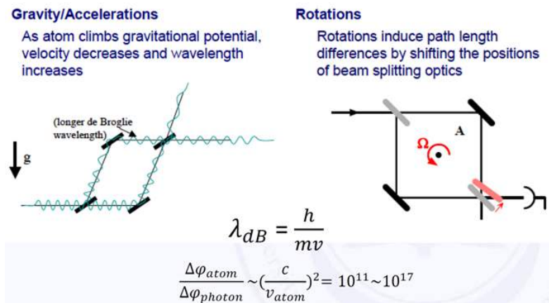
Figure 111: How cold atom interferometry works to measure both gravity, accelerations and rotations. Source: [1203].
