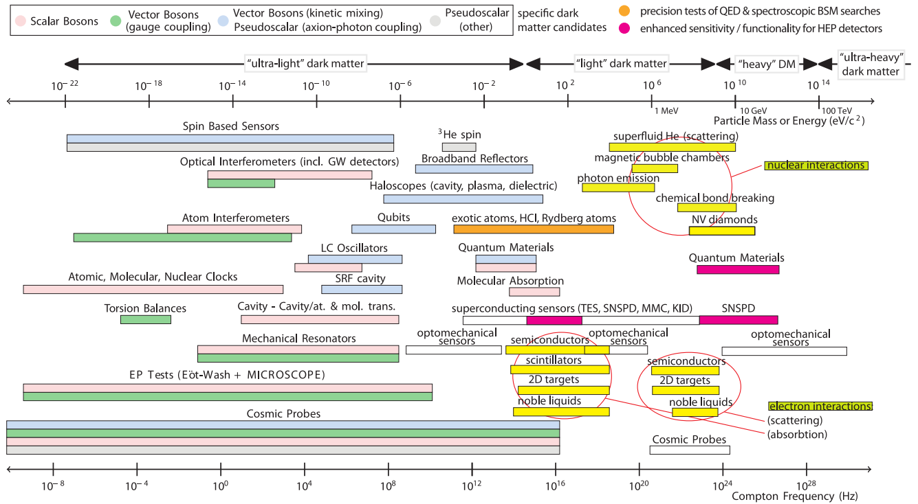
Figure 178: The various quantum sensors used for the search of dark matter. Source: [1605].
