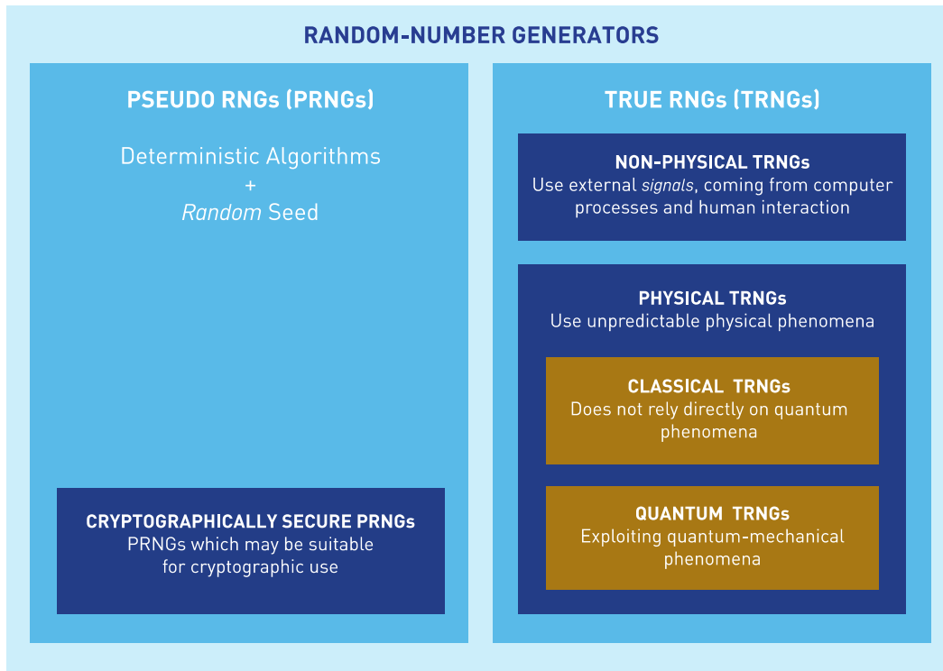
Figure 25: Taxonomy of random numbers generators. Source: [198].
