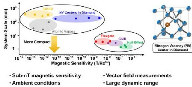
Figure 130: Magnetometers comparison. Source: [1292].
