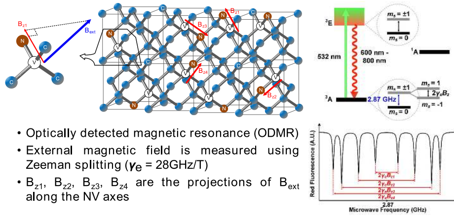
Figure 133: The principle of using NV centers in magnetometers. Source: [1292].
