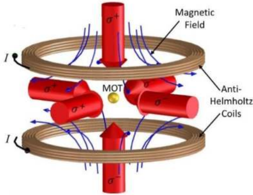
Figure 113: Typical Magneto-Optical Trap used to cool and confine neutral atoms. Source: [1231].
