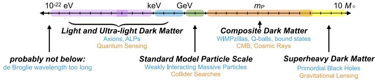
Figure 177: The energy levels of dark matter candidates. Source: [1602] which also positions very well the different quantum sensing techniques used in high-energy particle physics.
