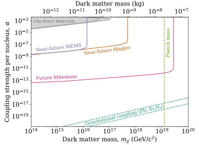
Figure 182: Dark matter sensitivity of the different sensor configurations investigated in [1601].
