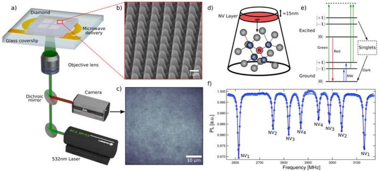
Figure 147: Widefield array of NV centers to improve their sensitivity, developed in Australia. Source: [1452].
