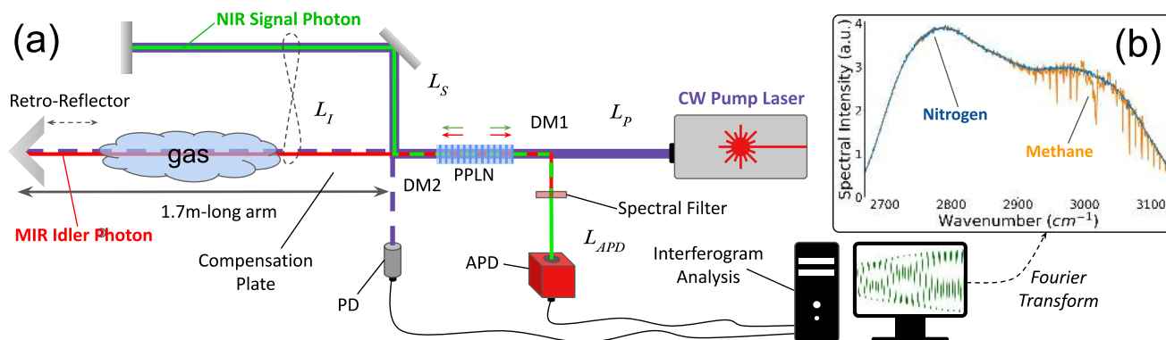
Figure 146: Quantum Fourier transform infrared (QFTIR) spectrometer uses a nonlinear Michelson interferometer. A periodically poled nonlinear crystal (PPLN) is pumped by a narrow-line CW pump laser, generating spectrally entangled signal and idler photons via SPDC (spontaneous parametric down-conversion). This conversion process occurs with low probability, either on the pump's first passage or its second passage, after all modes have traveled through the interferometer and have been reflected back into the crystal. The overlap of all beams in the interferometer erases the which-way information, making it impossible to know whether the photons were emitted on the first or second passage. By induced coherence, interference appears in the signal channel when the idler path length changes. A classical Fourier transform of the resulting interferogram obtained by the APD (avalanche photodiode) readout gives the spectral intensity of the idler photon, including the absorption of a sample placed on its path. Source: [1429].
