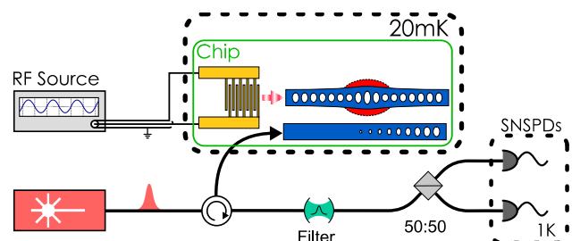
Figure 88: QPhox transduction architecture using an opto-electromechanical chip for the transduction of microwave photons to optical photons. Source: [1037].
