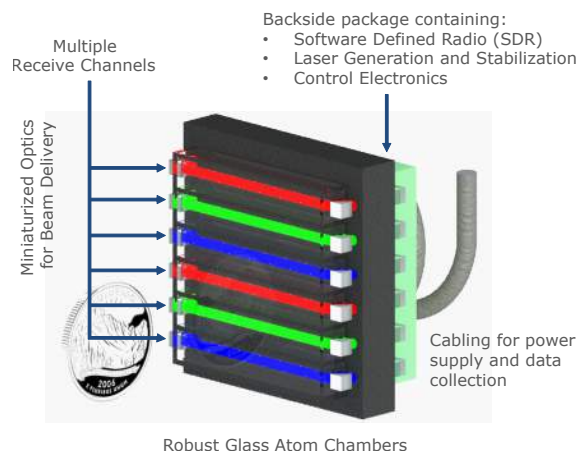
Figure 141: Infleqtion’s SqyWire vapor atom-based RF sensor. Source: [1388].
