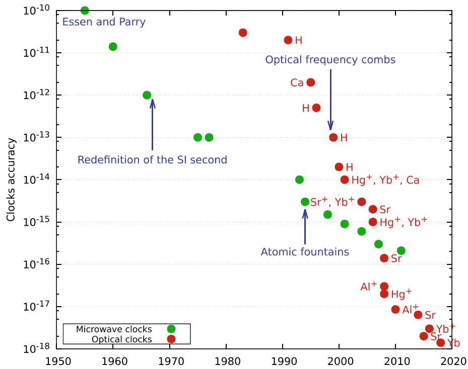
Figure 120: How quantum clock accuracy evolved over time. A recent multi-ion clock reached a systematic fractional frequency uncertainty of about 5 \times 10^{-19} in 2026 [1247]. Chart source: [1248].
