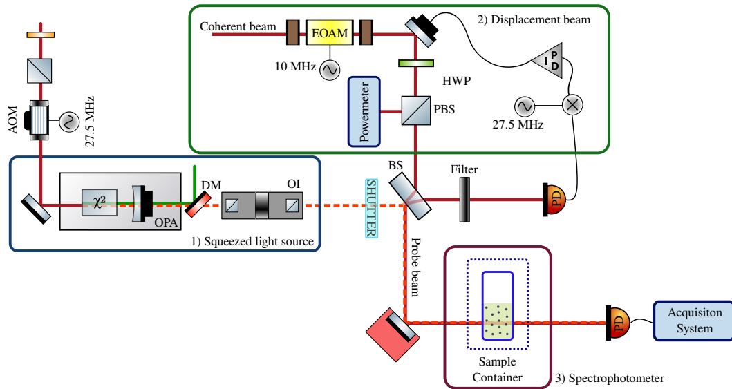
Figure 155: A quantum photometry experimental setup for an early bacterial detection. The three parts are a squeezed light source, a displacement beam module and a photometer. OPA: Optical Parametric Amplifier, DM: Dichroic mirror, OI: Optical isolator, HWP: Half-wave plate, PBS: Polarizing beam-splitter, BS: Beam-splitter, PD: Photodetector, EOAM: Electro-optic modulator, AOM: Acoustic optical modulator. Source: [1469].
