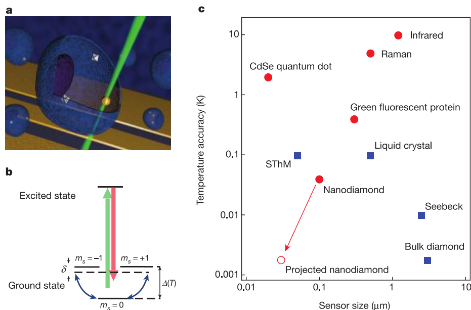
Figure 173: Hybrid thermometers associating NV centers and classical magnetic nanoparticle thermometers can be used to measure temperature within biological cells. Source: [1563].
