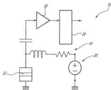
Figure 99: Electron-tunneling QRNG concept used by Quantum eMotion.
