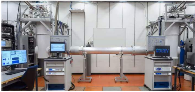
Figure 66: ETH Zurich 5-meter cryogenic microwave link. The waveguides were cooled to below 20 mK. Source: [812].
