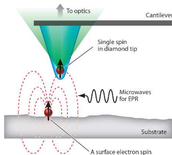
Figure 150: Typical NV center in a diamond tip for various imaging applications. Source: [1460].
