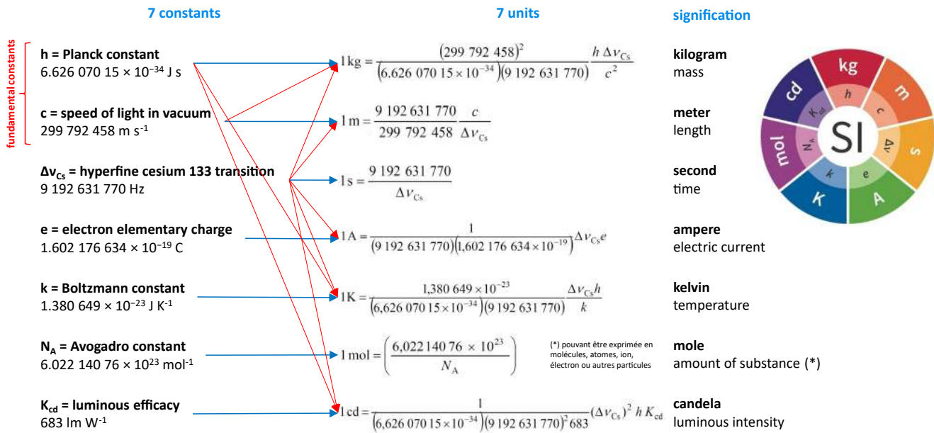
Figure 107: Reconstruction of the SI constants, units and their signification. Sources: © Olivier Ezratty, 2021-September 2026, and [1149].
