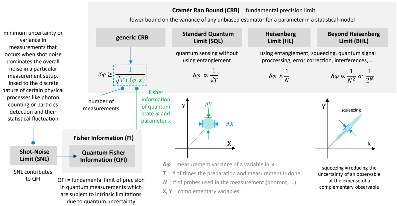
Figure 109: Mapping of the various quantum measurement limits. © Olivier Ezratty, 2023.
