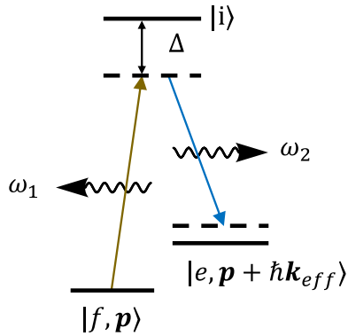
Figure 115: Atomic states of a ^{87}\text{Rb} atom and stimulated Raman transitions induced by counter propagating laser beams. [1237].
