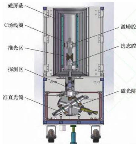
Figure 117: NIM-TF3’s atomic clock from the National Institute of Metrology of China is 1.5 meter tall. Source: [1242].
