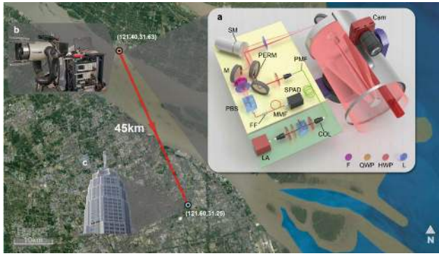
Figure 170: A test of quantum LiDAR with a range of 45 km in China in 2019. Sources: [1424, 1550].
