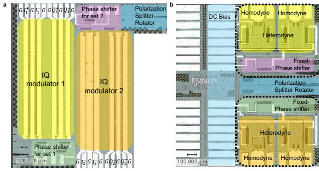
Figure 56: An example silicon-based chip for QKD distribution. Source: [548].
