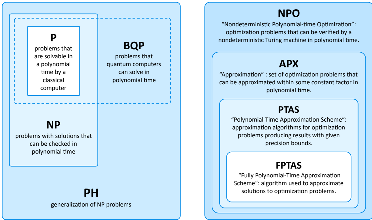
Figure 86: Schematic relation of BQP to selected classical complexity classes. NPO, APX, PTAS and FPTAS are optimization or approximation notions different from decision classes on the left. © Olivier Ezratty, 2022–September 2026.
