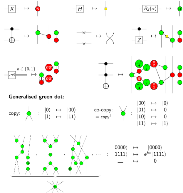
Figure 95: ZX calculus graphical language key operations. Source: [1529].
