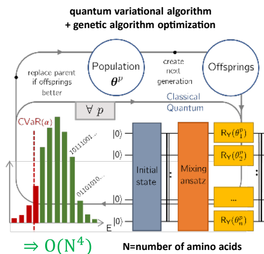
Figure 54: Hybrid classical and quantum lattice-model approach to protein folding. The 10-amino-acid Angiotensin instance was represented with 22 qubits in simulation, while the paper's smaller 7-amino-acid instance was run on IBM hardware. This is not directly comparable to AlphaFold 3, which solves a different classical structure-prediction task. Source: [839].
