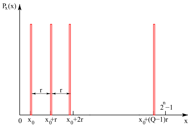
Figure 40: These two figures above illustrate the phase register before and after the inverse QFT in a textbook Shor order-finding circuit. Before the inverse QFT, the amplitudes are supported on basis states separated by the period r , with an offset x_0 . The inverse QFT maps this periodic structure to peaks near integer multiples of 2^m/r , where m is the number of phase-register qubits.
