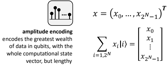
Figure 18: Amplitude encoding creates a normalized state whose computational-basis amplitudes encode a vector. A generic arbitrary target may be entangled and generic exact state preparation has exponential gate complexity in the number of qubits. © Olivier Ezratty, 2021-2026.
