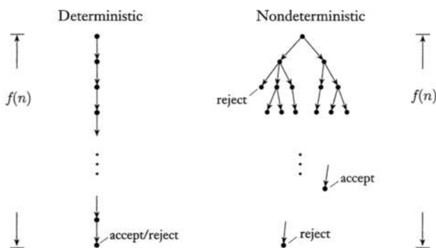
Figure 75: Deterministic and nondeterministic Turing machines.
