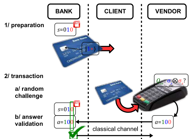
Figure 195: A quantum money scheme. Source: [2877].
