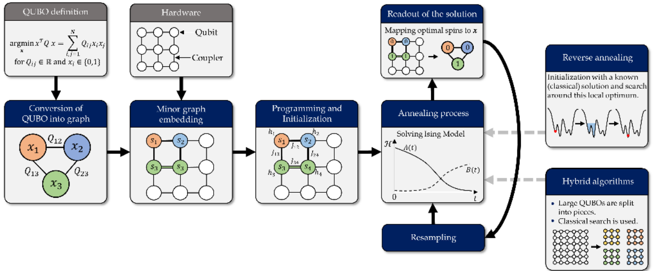
Figure 67: A quantum annealing process taking the example of an optimization problem encoded in a QUBO problem and a related graph. The graph is automatically mapped to a graph compatible with the qubit topology of a D-Wave QPU through the process of “minor graph embedding”. The graph is then encoded in the system with an initialization of the qubit weights and connections. The annealing process creates a transverse magnetic field that sets the qubits value in a superposed state and progressively removing this field, which implements the annealing process, converging the qubit towards their optimum value minimizing the total system energy. Then the qubits are read out. The process is repeated several times and the result values averaged. Variations involved reverse annealing when the graph initialization uses a known classical solution and the annealing process helps find a better solution around it, and hybrid algorithms where large QUBO problems are split classically into smaller QUBO problems. Source: Sheir Yarkoni et al. in [1229]. Added in 2023.
