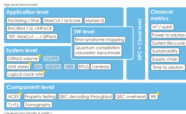
Figure 141: From low-level to high-level benchmarking proposals. Source: [2039].
