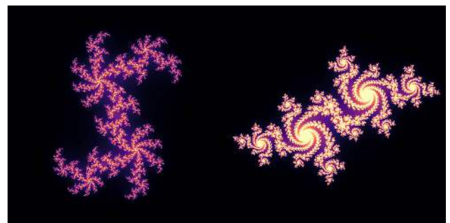
Figure 200: Wiktor Mazin fractal example. Source: [3095].
