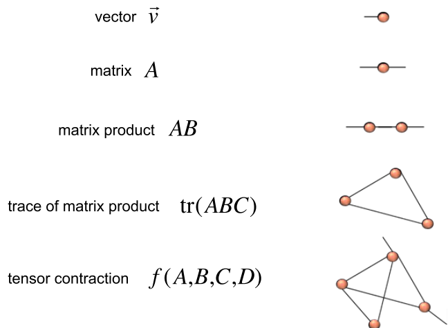
Figure 87: Basics of tensor networks operations. Source: [1452]
