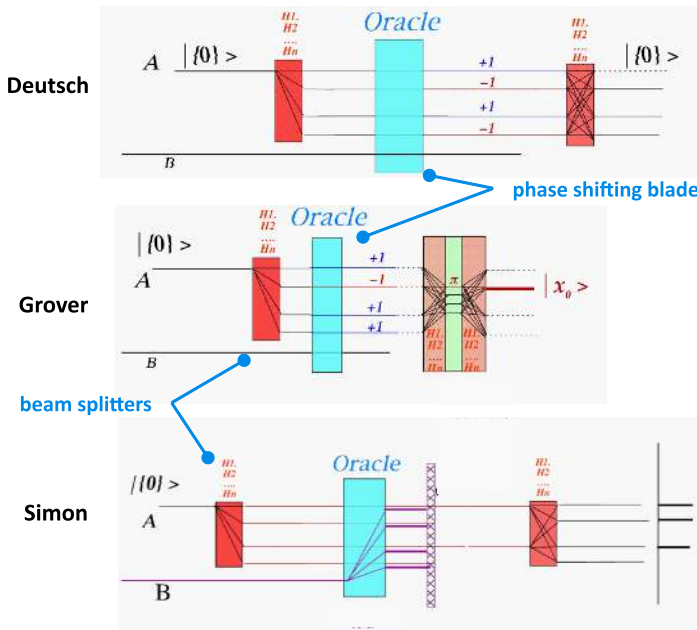
Figure 36: Quantum algorithms explained with interferences when implemented with quantum optics. Source: Serge Haroche, Chaire de Physique quantique. 2001-2002. 8 th lesson, February 26 th , 2002.
