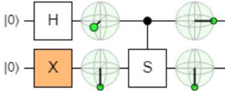
Figure 21: A two-qubit phase kickback shown using the Quirk emulator.
