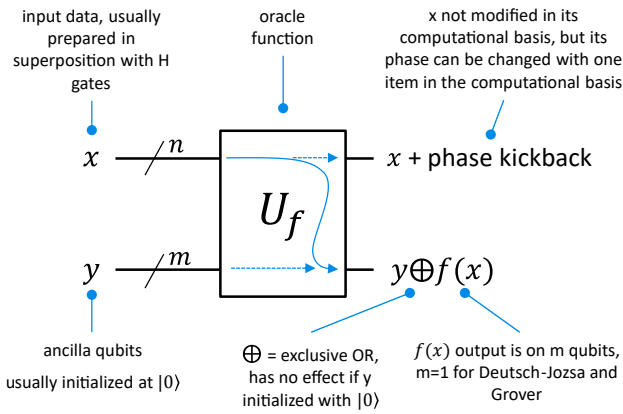
Figure 20: How an oracle function is used in an algorithm, in complement of a phase kickback. © Olivier Ezratty, 2021.
