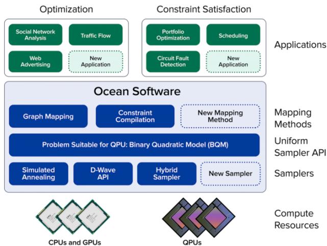
Figure 122: D-Wave's Ocean software architecture. The image is a conceptual view. Current software package names and versions are available in the Ocean documentation. Source: D-Wave.
