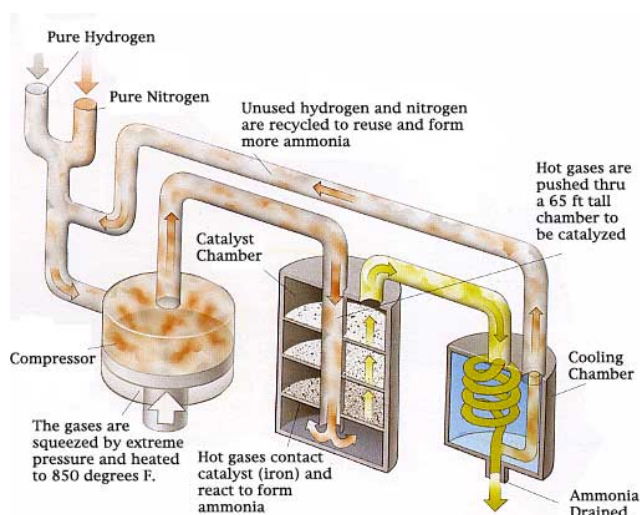
Figure 175: The usual Haber-Bosch process. Source: [2540].
