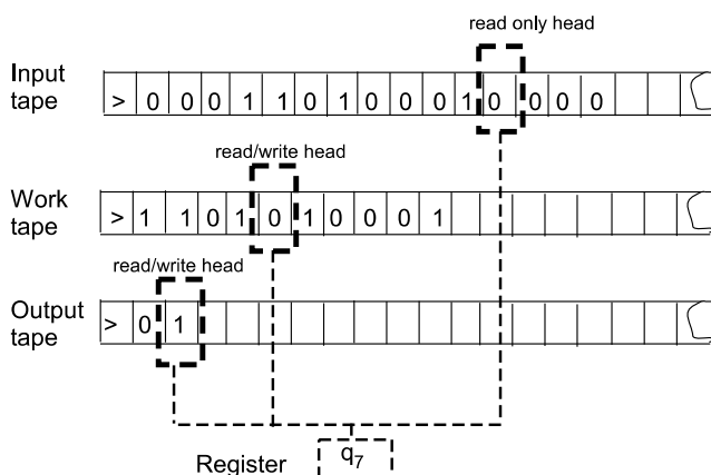
Figure 74: The Turing machine. Source: [1327].
