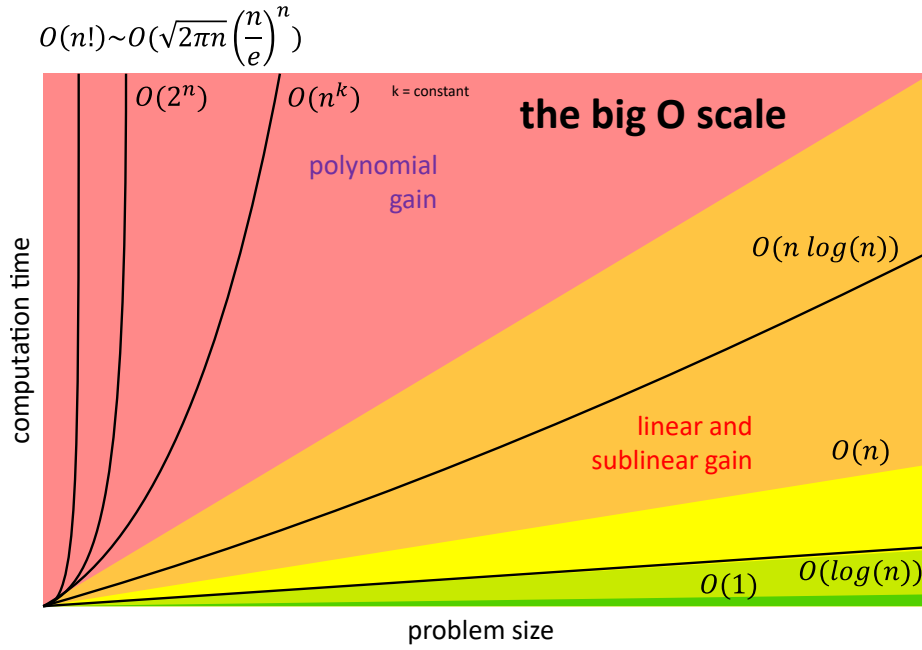
Figure 69: Another view of common asymptotic growth functions. The factorial growth n! is asymptotically described by Stirling's formula, n! \sim \sqrt{2\pi n}(n/e)^n . Such a running time grows faster than c^n for every fixed constant c , but this property alone does not determine what quantum speedup is possible for a particular problem. Source: Wikipedia, reformatted with additions by Olivier Ezratty, © 2022-2026.
