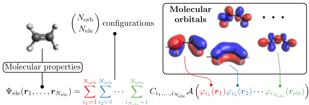
Figure 167: Example of a butadiene electronic wavefunction \psi_{ele} . In full configuration interaction within a chosen orbital basis, it is expanded as a linear combination of Slater determinants built from molecular spin orbitals. Source: [2420]. Added in 2023.
