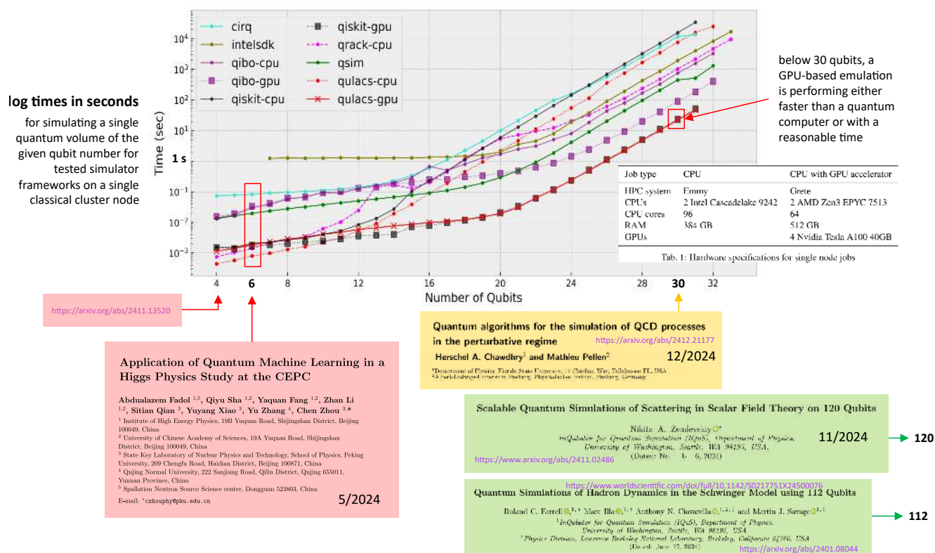
Figure 204: How HEP quantum computing simulations have grown in time to overcome the 100 physical qubit barrier. Sources for 3 qubits [3219, 3220], 4 qubits [3221], 6 qubits [3222], 30 qubits [3223], 112 qubits [3224] and 120 qubits [3225]. The above chart shows the time spent to emulate classically an equivalent circuit with a depth and breadth of N qubits, the best results being obtained with GPUs [1685]. For the circuits and systems measured here, GPU-based simulation compares well with the quantum runs up to about 30 qubits, in relative computing time and in seconds. This is specific to the tested circuit families, fidelities and outputs, and the configurations compared do not have matching prices, latency or amortization. © Consolidation by Olivier Ezratty, January 2025.
