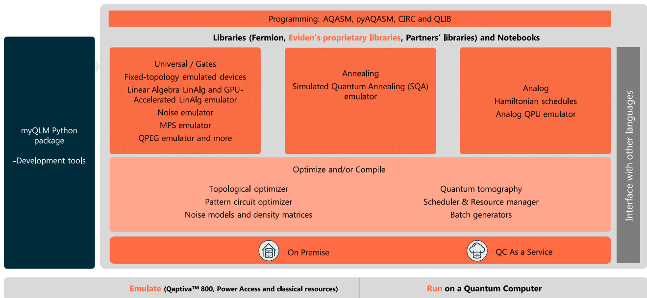
Figure 134: Bull software platform. Source: [1867]. The diagram predates Qaptiva HPC, launched in November 2024, and the current Qaptiva portfolio described in the text.
