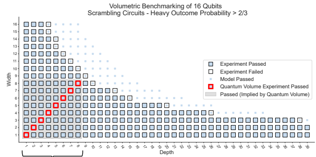
Figure 144: How is/was IBM's 2017 and 2019 quantum volumes calculated. © Olivier Ezratty, 2021-September 2026.
