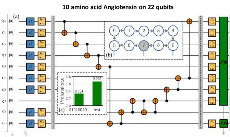
Figure 54: Hybrid classical and quantum lattice-model approach to protein folding. The 10-amino-acid Angiotensin instance was represented with 22 qubits in simulation, while the paper's smaller 7-amino-acid instance was run on IBM hardware. This is not directly comparable to AlphaFold 3, which solves a different classical structure-prediction task. Source: [839].
