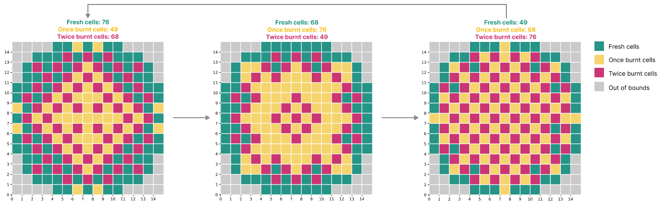
Figure 184: Source: a prototype solution to solve the nuclear plants in-core fuel management problem. It is a QUBO solution made for quantum annealers but is not yet in a quantum advantage regime. Source: [2759].
